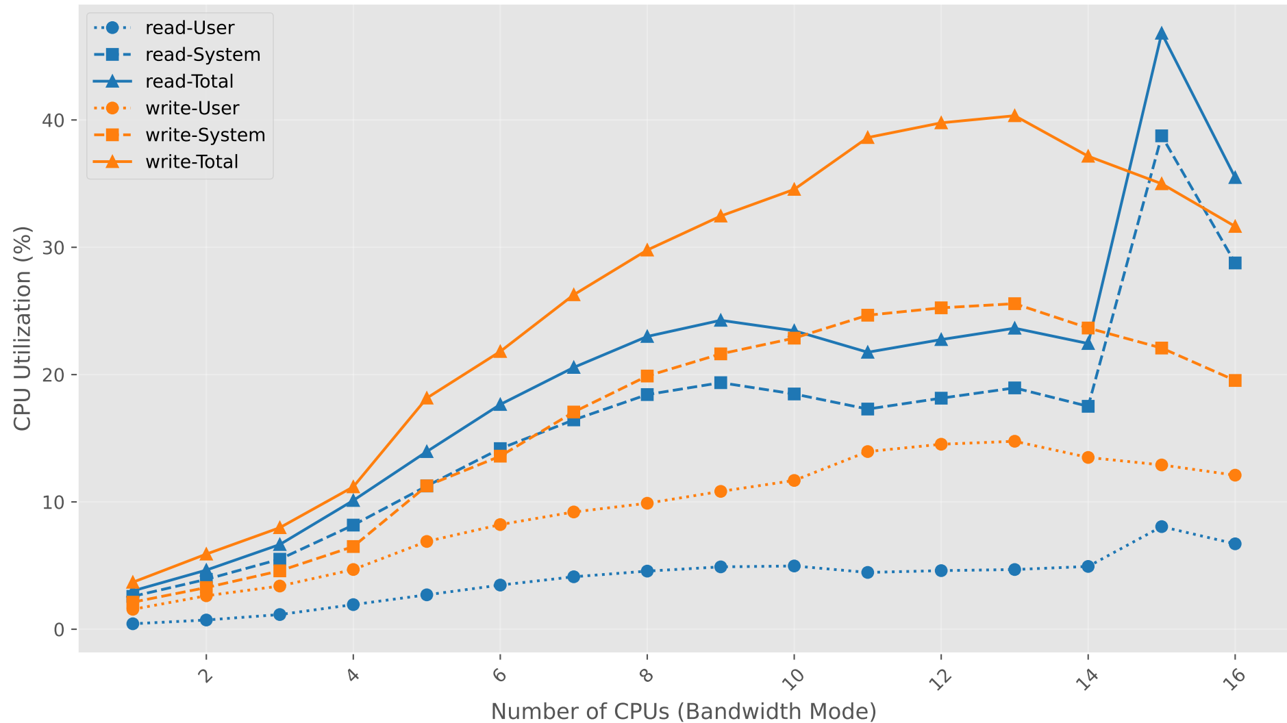
CPU Total vs Number of CPUs (Bandwidth Mode)
